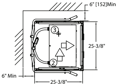
Corner Configuration
