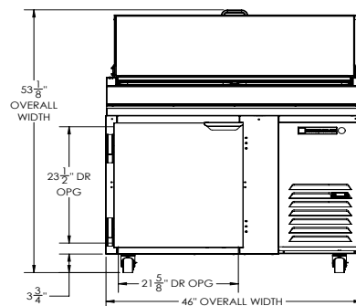
ELEVATION VIEW
