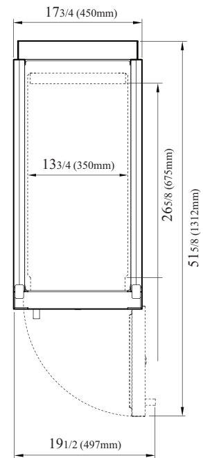
TOP VIEW
