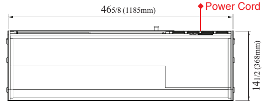
SAS-50R-N
