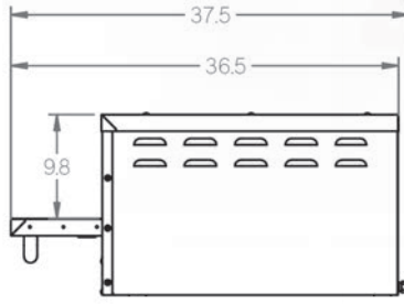
SIDE VIEW (OPEN DOOR)
