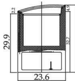
TSD-47CF/TSD-60CF SIDE VIEW
