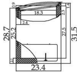
TSD-35CF SIDE VIEW
