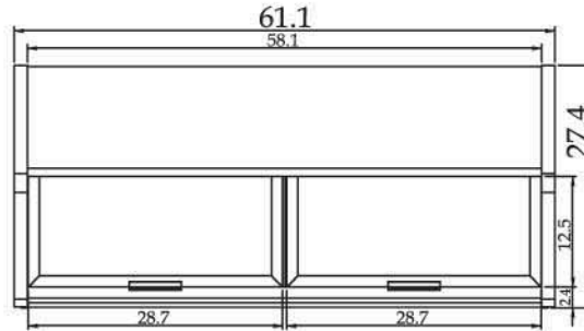
TGF-13F-PLAN VIEW
