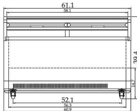
TGF-13F-FRONT VIEW
