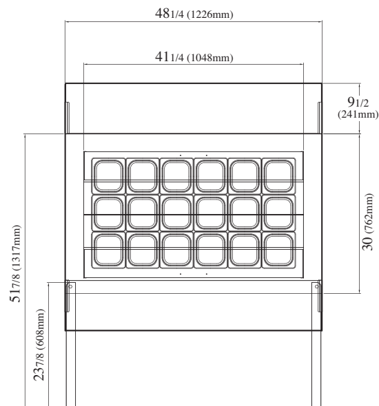
PLAN VIEW
